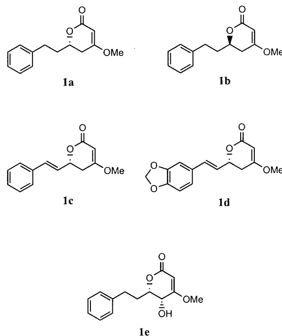
Figure 1. Important kavain derivatives.
