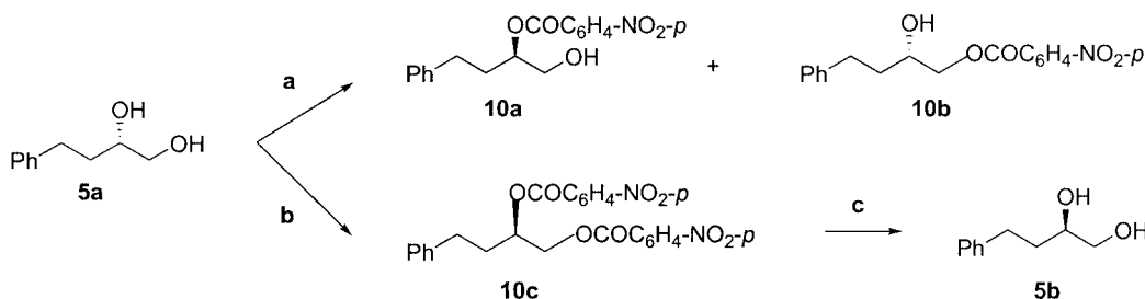
Scheme 2. Conditions and reagents: (a) \text{PPh}_3 (1 equiv.), DIAD (1 equiv.), p\text{-NO}_2\text{C}_6\text{H}_4\text{COOH} (1 equiv.), THF, room temp., 2 h; (b) \text{PPh}_3 (2 equiv.), DIAD (2 equiv.), p\text{-NO}_2\text{C}_6\text{H}_4\text{COOH} (2 equiv.), THF, room temp., 2 h; (c) catalytic Na, MeOH, room temp., 1 h.
