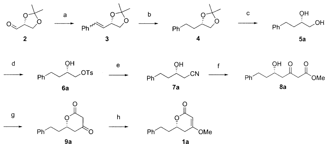
Scheme 1. Conditions, reagents and yields: (a) [\text{PhCH}_2\text{Ph}_3\text{P}]\text{Br} (1.0 equiv.), n\text{BuLi} (1.0 equiv.), THF, 0 °C, 2 h, 80%; (b) \text{H}_2 , 10% Pd-C, MeOH, room temp., 8 h, 98%; (c) 2 M HCl, MeOH, 1 h, room temp., 97%; (d) TsCl (1.1 equiv.), dry pyridine, ice-salt bath (−15 °C), 12 h, 75%; (e) KCN (1.5 equiv.), room temp., 12 h, 89%; (f) \text{BrCH}_2\text{COOMe} (5 equiv.), activated zinc (10 equiv.), ultrasound, THF, 5 h, 50 °C, 69%; (g) Catalytic amount of p -toluenesulfonic acid, \text{CH}_2\text{Cl}_2 , room temp., 2 h, 84%; (h) \text{Me}_2\text{SO}_4 (2 equiv.), \text{K}_2\text{CO}_3 (2 equiv.), acetone, room temp., 12 h, 86%.
